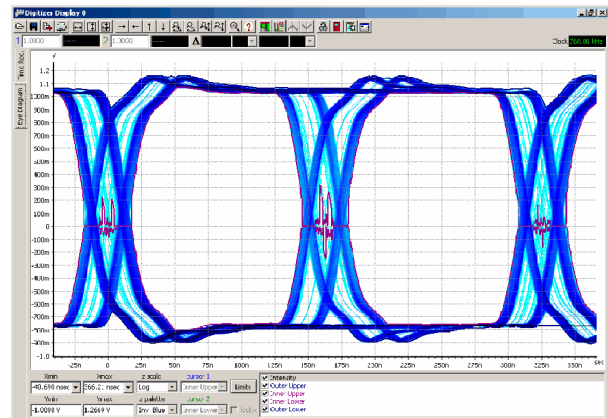
Eye diagram
